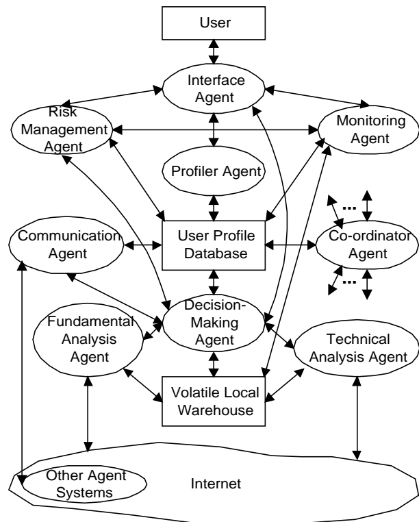
Figure 1. MASST Framework
