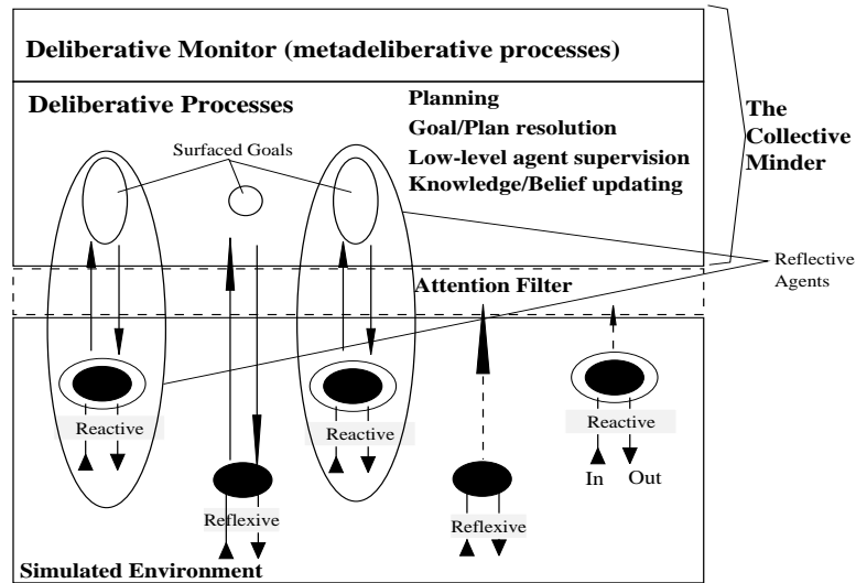
Fig. 1. The different levels of agency in the collective minder scenario.
