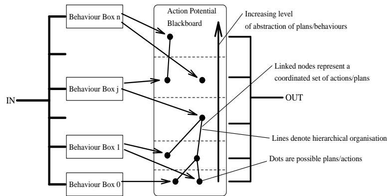
Fig. 4. Hybrid Behaviour-Based Architecture (with an action potential blackboard)
