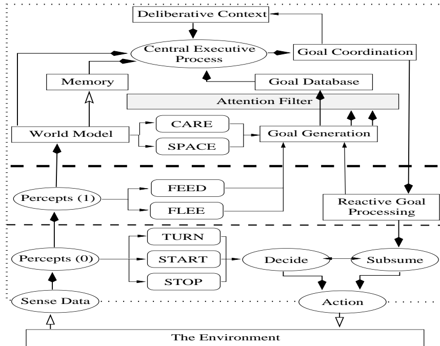
Fig. 5. A hybrid subsumption architecture for simple agents.
